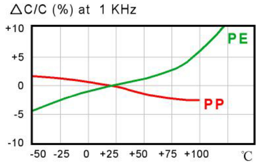
Temperature Characteristics
