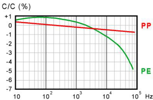
Frequency Characteristics
