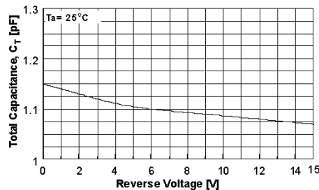
Figure 6. Total Capacitance
