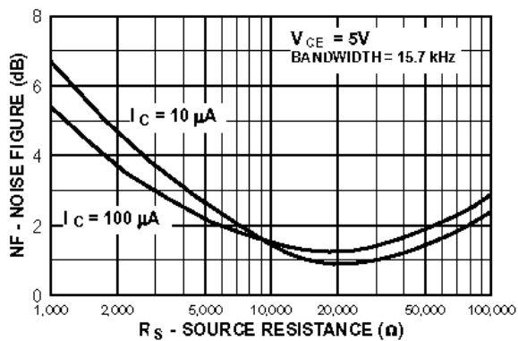
Figure 9. Wideband Noise Frequency vs Source Resistance
