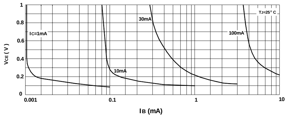
Collector Saturation Region
